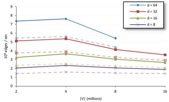
Fig. 12. Multi-GPU sensitivity to graph size and average out-degree for uniform random graphs using four C2050 processors. Dashed lines indicate predecessor labeling variants.
