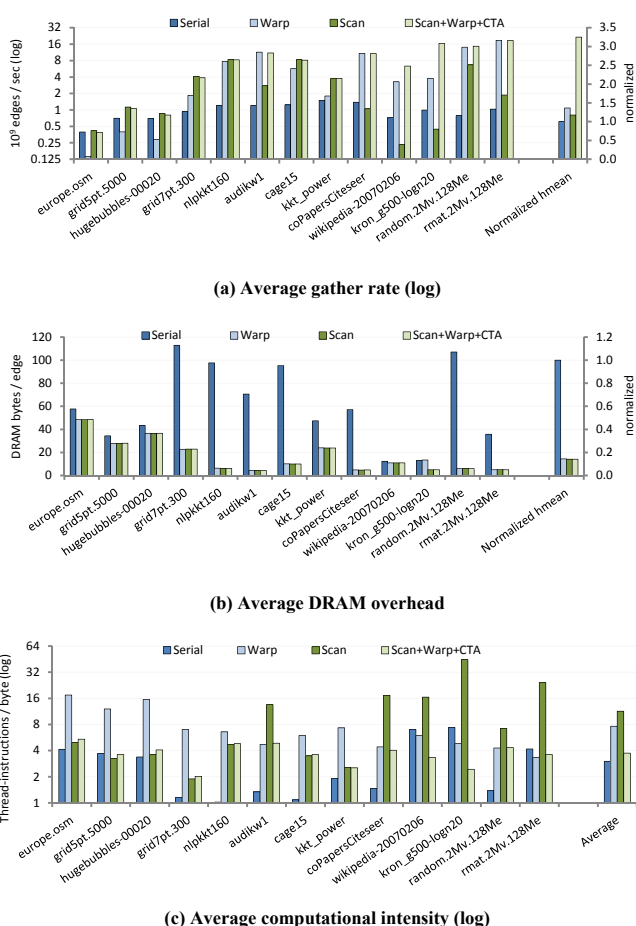
Fig. 5. Neighbor-gathering behavior. Harmonic means are normalized with respect to serial-gathering.
